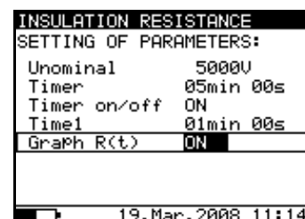
Fig. 14. Set-up menu in Insulation Resistance measurement
