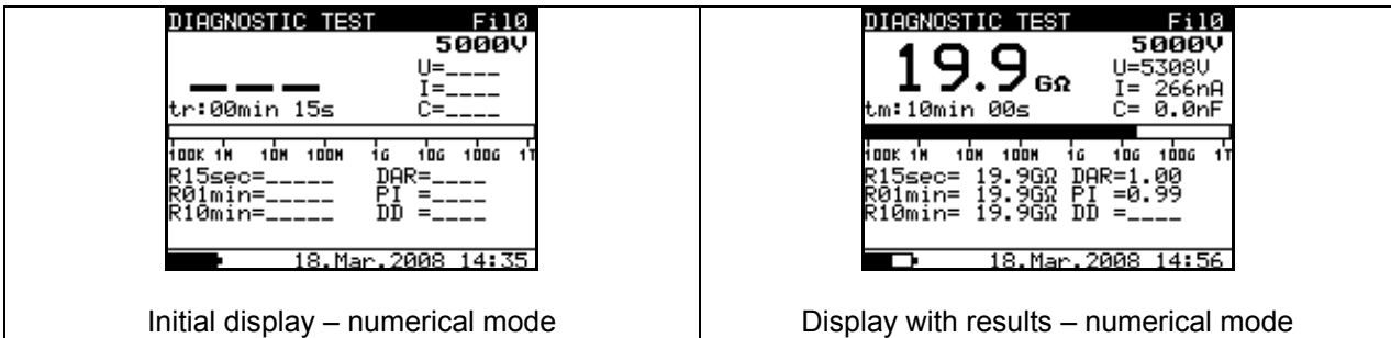
Fig. 16. Diagnostic test display states - Graph R(t) disabled
