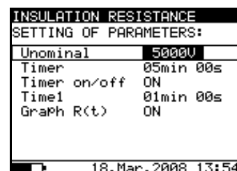
Fig. 13. Set-up menu in Insulation Resistance measurement
