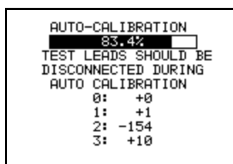
Fig. 4. Auto-calibration state
