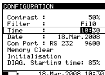
Fig. 6. Configuration state
