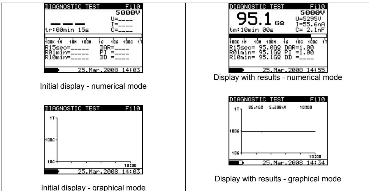
Fig. 17. Diagnostic test display states - Graph R(t) enabled
