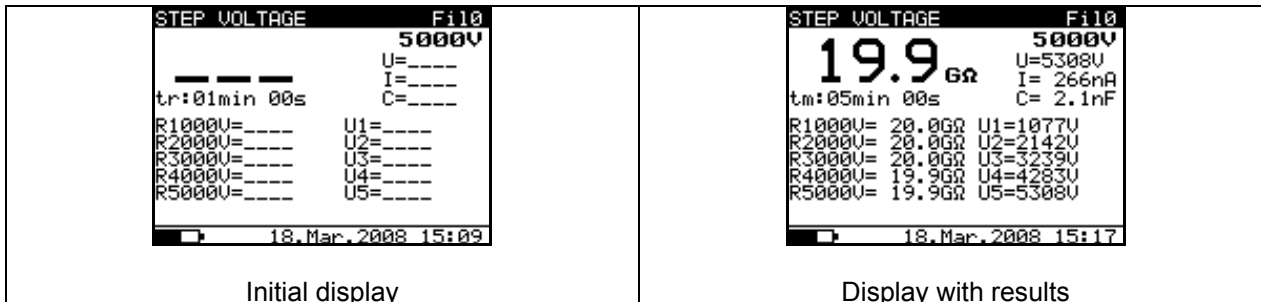
Fig. 22. Step Voltage function display states- Graph R(t) disabled
