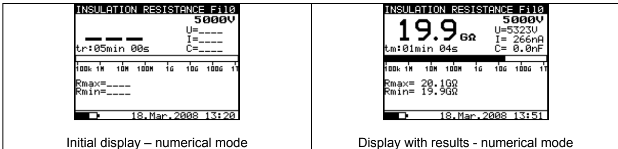
Fig. 11. Insulation Resistance function display states - Graph R(t) disabled
