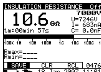
Fig. 31. Storage operation menu
