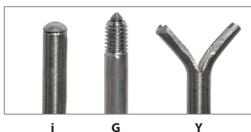
Art.-no. 89312 i semicircular electrode (standard) Art.-no. 89314 G peaked electrode with M5-thread Art.-no. 89316 Y bifurcated electrode
