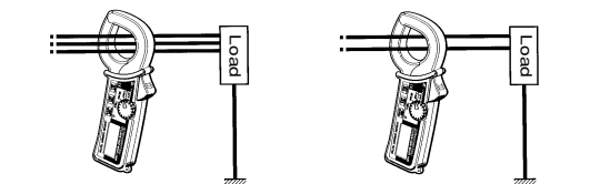
Fig. 2 Measuring out of balance leakage current
