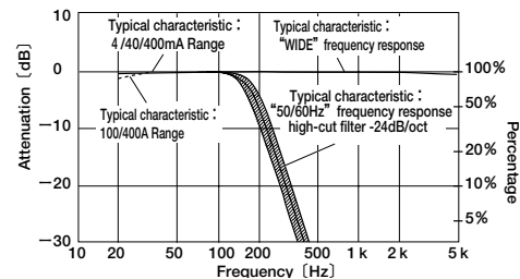
Fig. 3 Model 2432/2433 Frequency Characteristic
